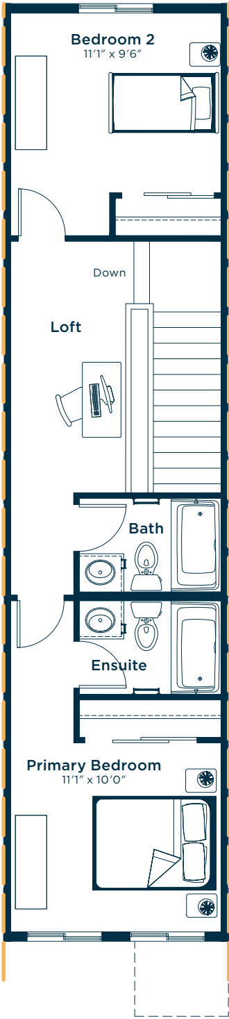
SECOND FLOOR 591 SQ.FT.
