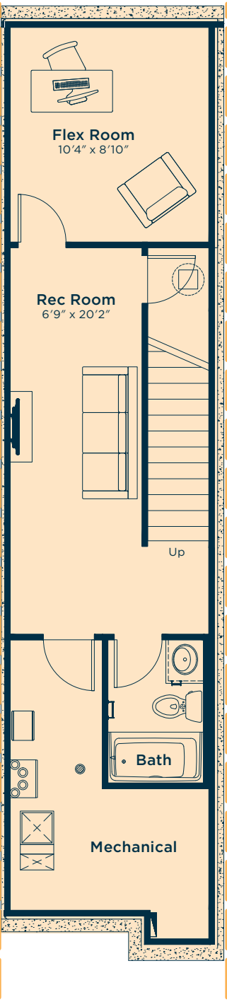
Develop the basement below with an flex room, rec room and bath 354 SQ.FT.
