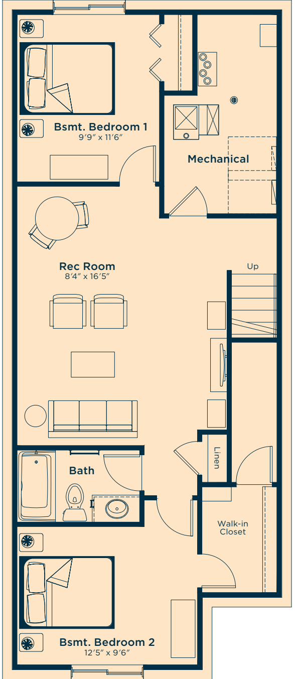
Develop the basement below with two bedrooms, rec room and bath 678 SQ.FT.
