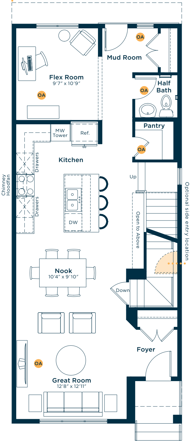
MAIN FLOOR 913 SQ.FT.
