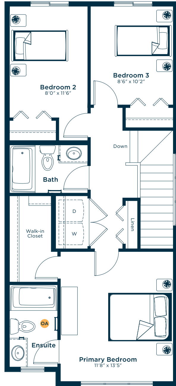
SECOND FLOOR 712 SQ.FT.
