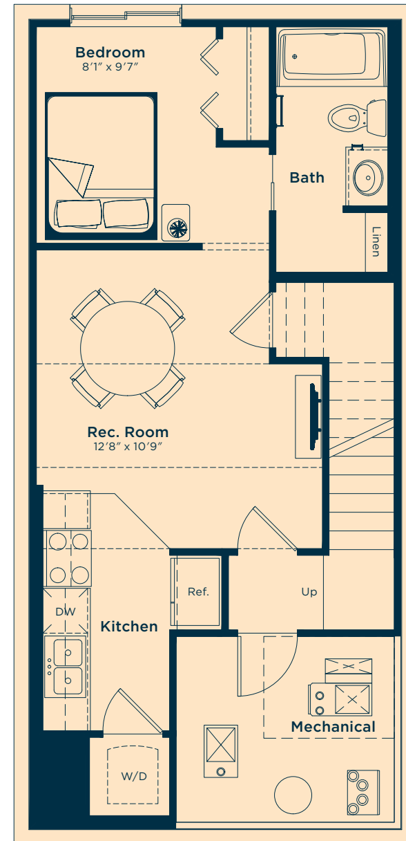
Develop a basement suite below with a bedroom, kitchen, rec room and bath 463 SQ.FT.
